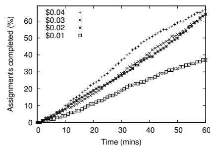
Figure 6: Completion (%): Vary Reward (100 HITs/Group, 5 Asgn/HIT)
