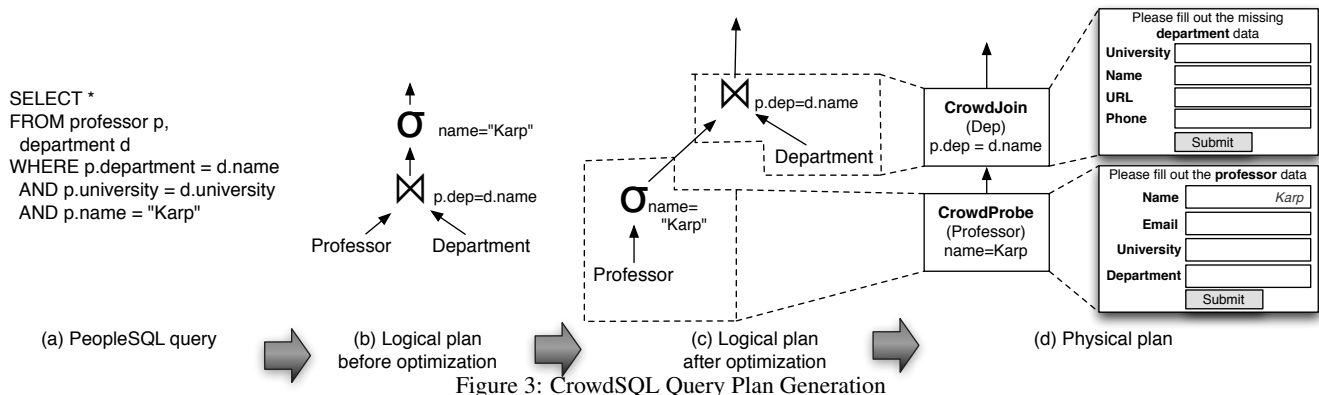
Figure 3: CrowdSQL Query Plan Generation
